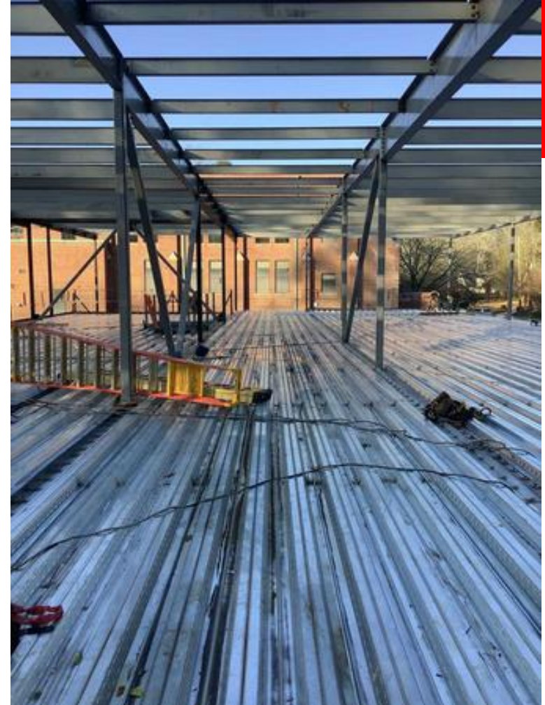
Second floor decking install
